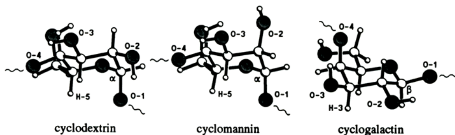
Fig. 2. Zoom of the mean monosaccharide units for the minimum energy structures in Fig. 1 as seen perpendicular to the cyclooligosaccharide mean plane. Due to the inclination of the pyranoid rings in respect to the macro ring, the \alpha -D-glucosyl and \alpha -D-mannosyl units are seen from their "bottom" sides (compare to the residue geometries in top right corner of the cyclohexaoside structures in Fig. 1), whereas the \beta -D-galactosyl residue (bottom left unit of cyclo [Gal \beta (1 \rightarrow 4)] 6 in Fig. 1) corresponds to the conventional depiction of a {}^4C_1 pyranose conformation.
