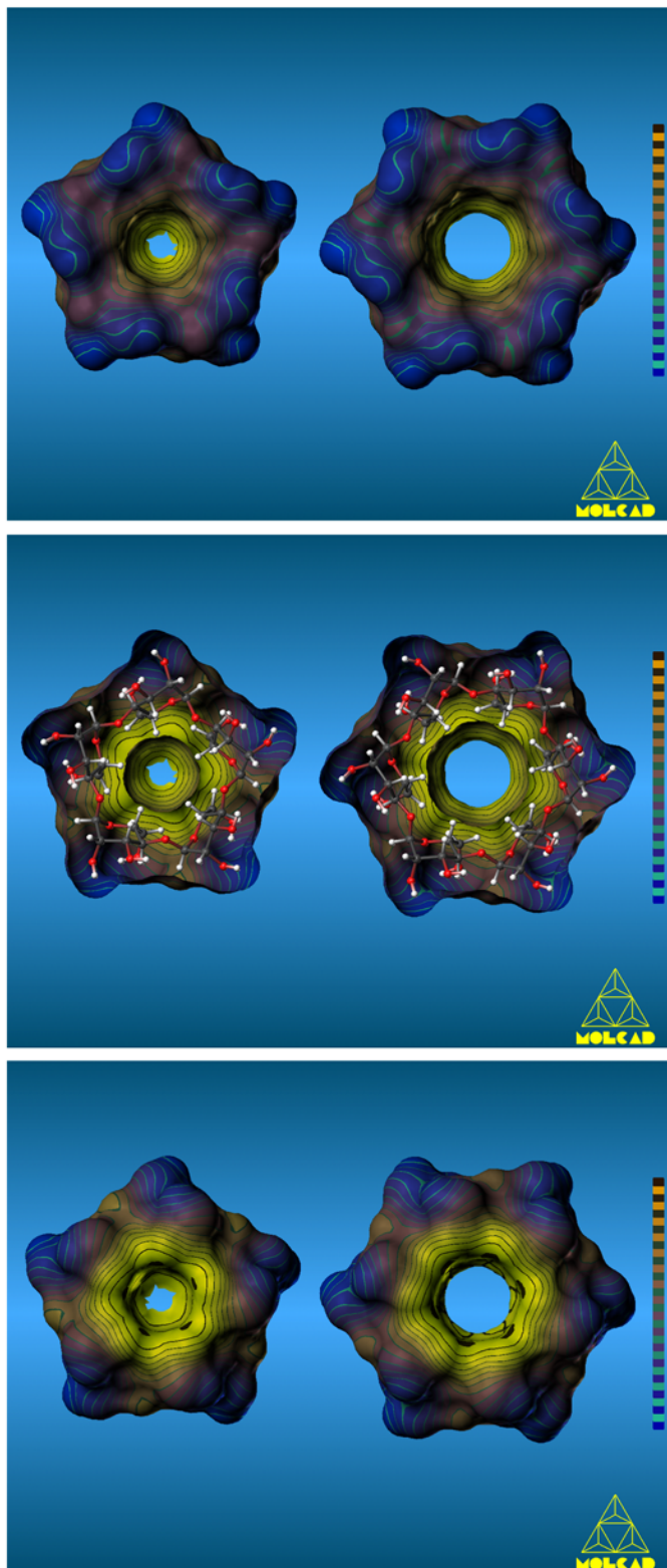
Fig. 5. MLPs of the cyclomannins 6 and 7 with five (left) and six (right) \alpha(1\rightarrow4) -linked mannose units, respectively; orientation of the molecules and mode of visualization as in Fig. 4.
