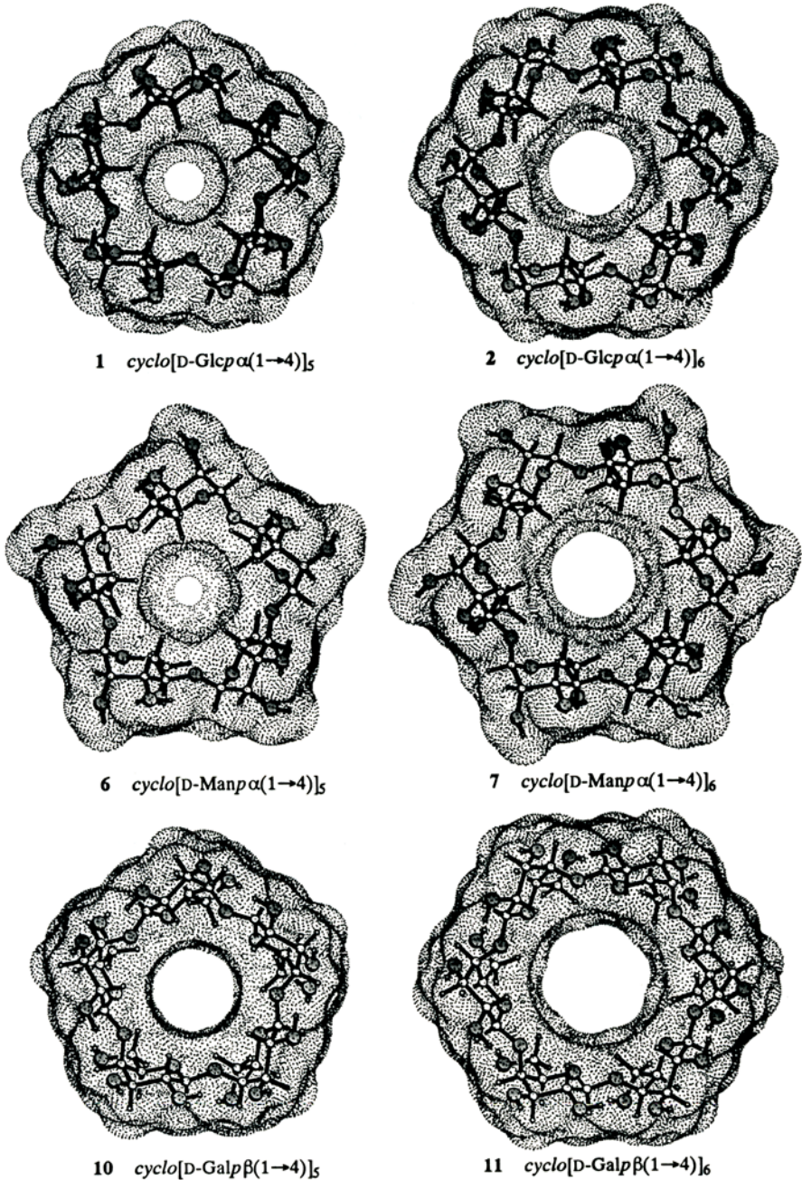
Fig. 1. Minimum energy structures (PIMM91) and contact surfaces in dotted form for the cyclodextrins (upper plots), cyclomannins (center), and cyclogalactins (lower row) containing five (left) and six-monosaccharide units (right column), respectively. Structures are shown perpendicular to the mean ring plane of the macrocycles and viewed through the large opening of the conically shaped molecules, i.e. the 2-OH / 3-OH side of the pyranoid rings points towards the viewer, and the primary \text{CH}_2\text{OH} groups away from him, towards the back.
