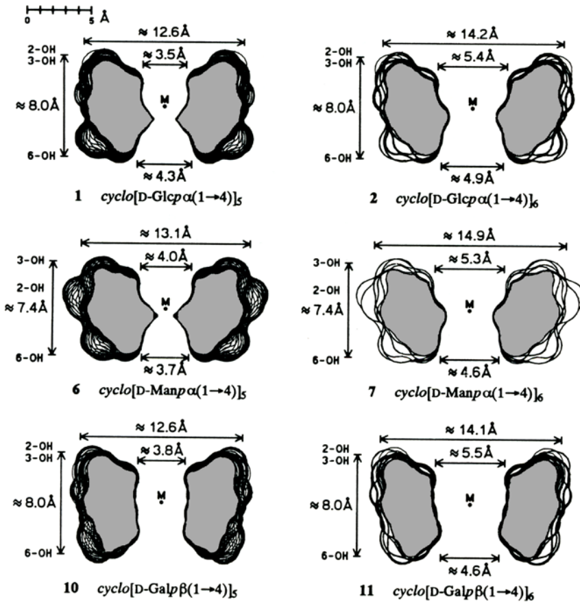
Fig. 3. Cross cut plots through the contact surfaces and approximate molecular dimensions of the (1→4)-linked cyclodextrins (1 and 2, top), cyclomannins (6 and 7, middle), and cyclogalactins (10 and 11, bottom). The contour lines result from successive 10° rotation steps around the geometrical center M. In each case, the larger opening (top side each) of the conically shaped molecules carries the secondary 2-OH and 3-OH at the torus rim, whilst the primary 6-OH groups are positioned at the opposite (bottom) side forming the rim of the smaller opening.
