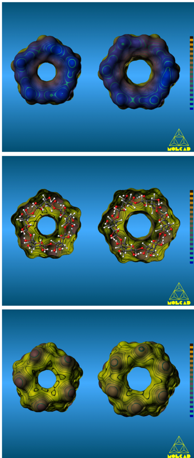
Fig. 6. MLPs of the \beta(1\rightarrow4) -cyclogalactins 10 and 11, composed of five (left) and six (right) galactose residues. Mode of viewing as in Fig. 4.
